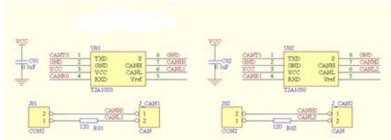
Figure 6 CAN bus section circuit diagram
